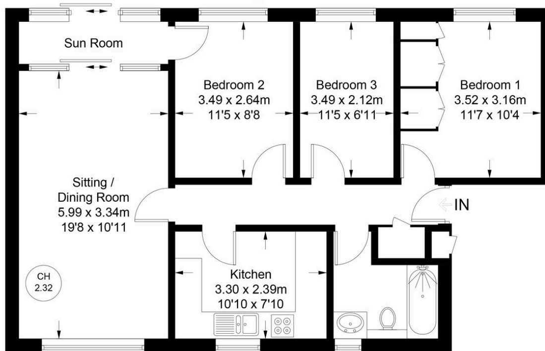
Ground Floor
