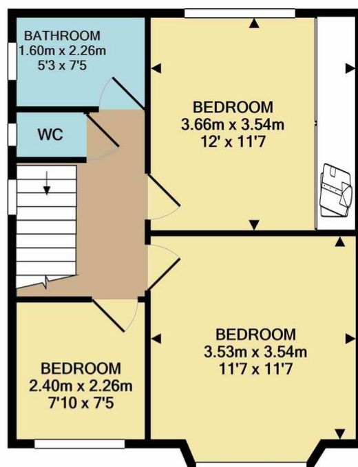
1ST FLOOR APPROX. FLOOR AREA 42.3 SQ.M. (456 SQ.FT.)
