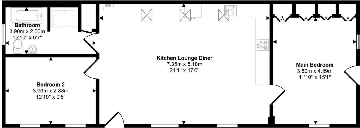
Floorplan
