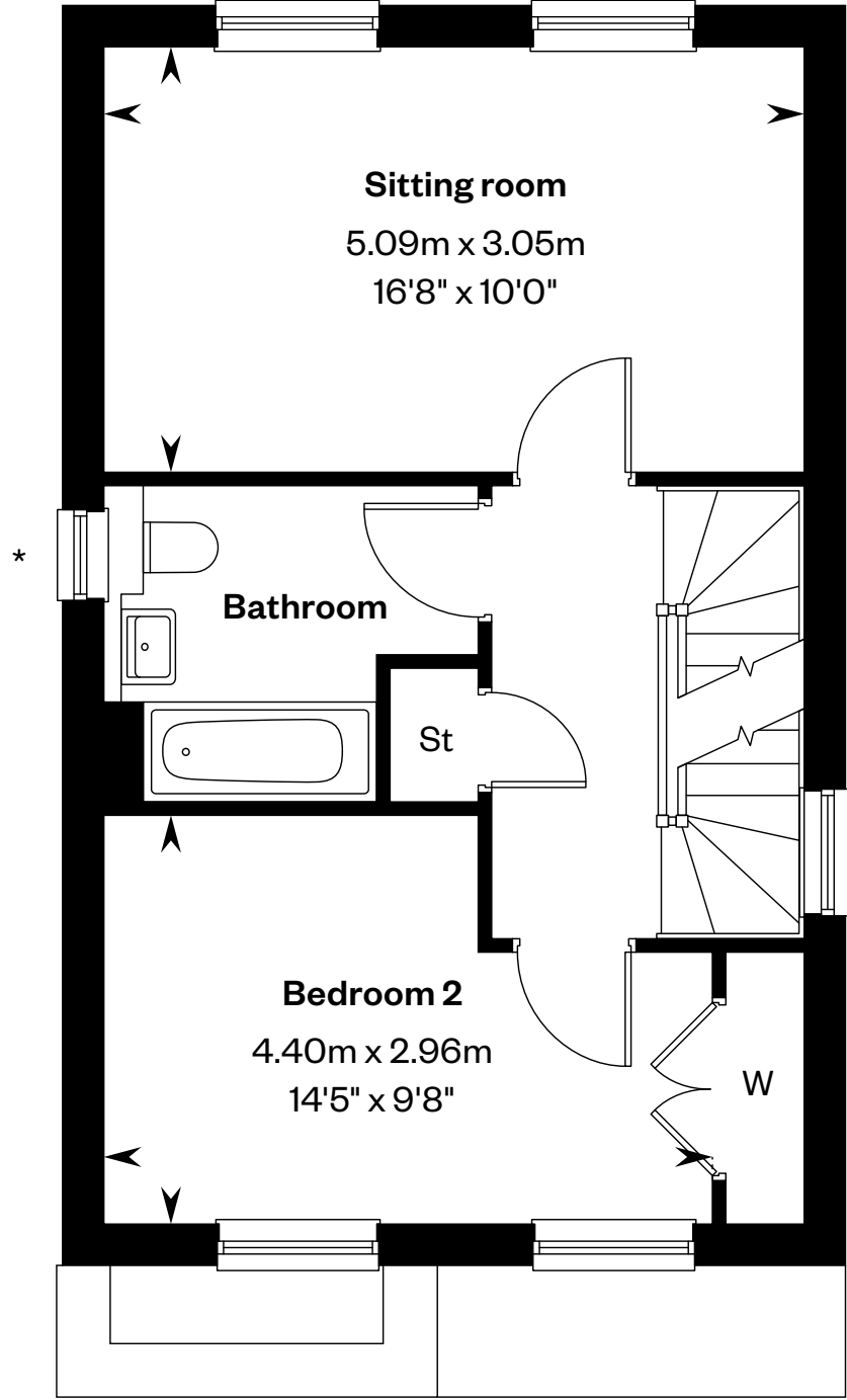
First floor
