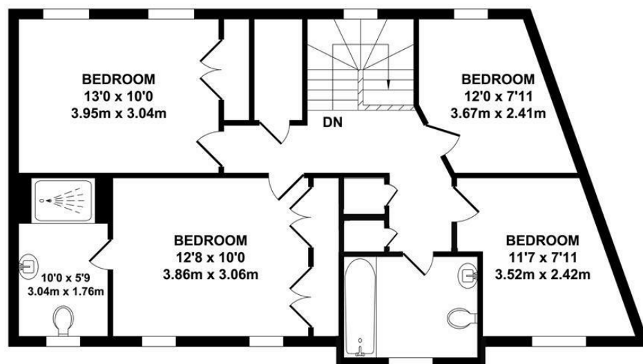
FIRST FLOOR APPROX. FLOOR AREA 747 SQ.FT. (69.40 SQ.M.)
