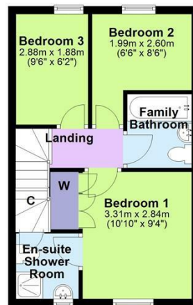
First Floor Approx. 34.0 sq. metres (365.5 sq. feet)
