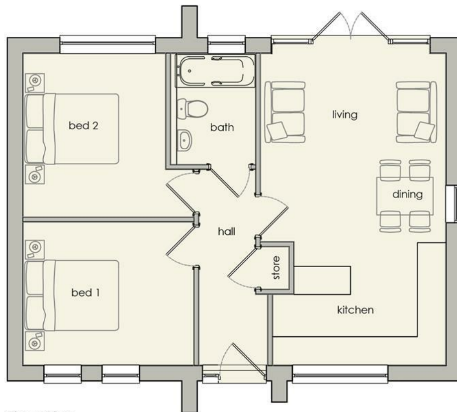
Floor Plan
