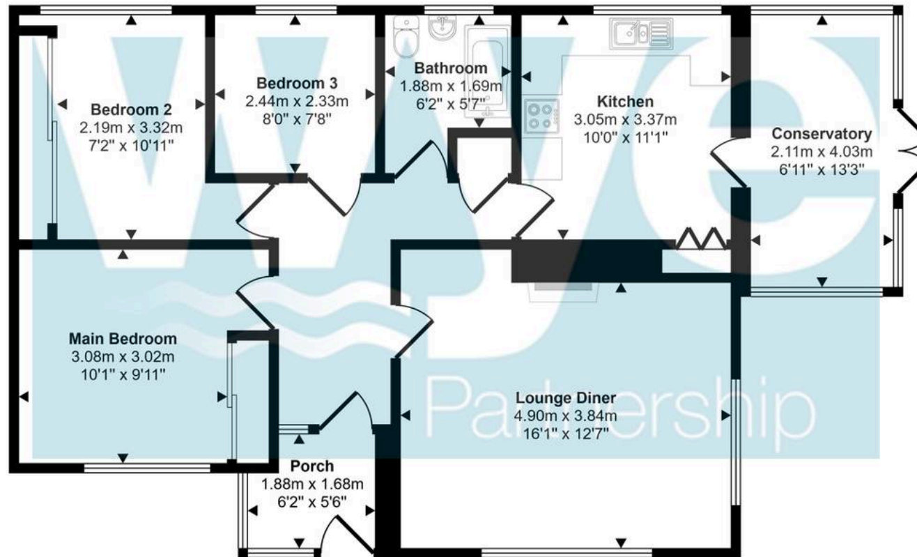
Floorplan
