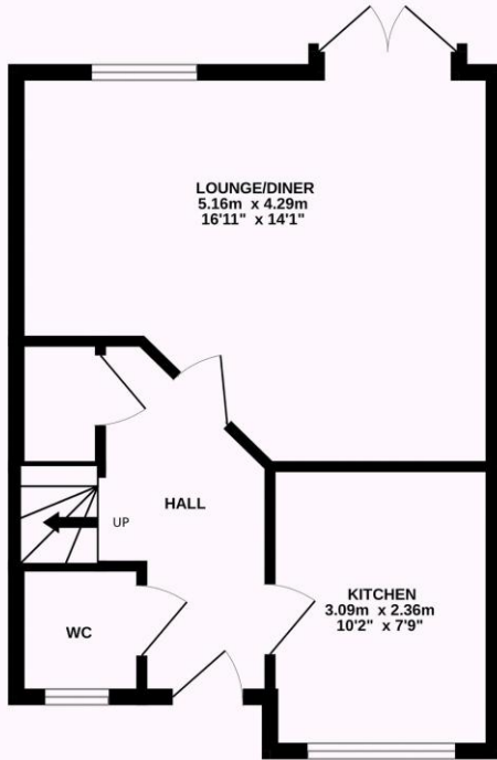
GROUND FLOOR 37.0 sq.m. (399 sq.ft.) approx.
