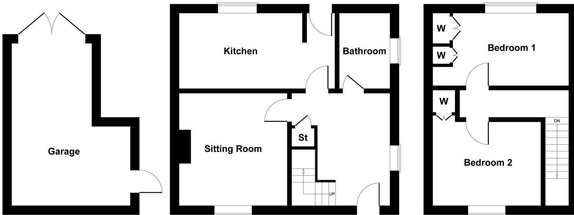
FIRST FLOOR
