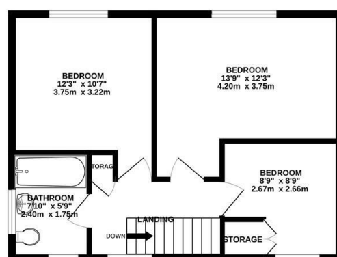
1ST FLOOR 442 sq.ft. (41.1 sq.m.) approx.
