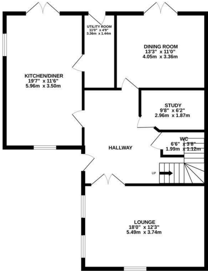
GROUND FLOOR 896 sq.ft. (83.2 sq.m.) approx.
