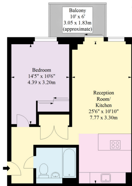
Third Floor
