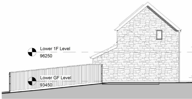
1 North East Elevation 1 : 100
