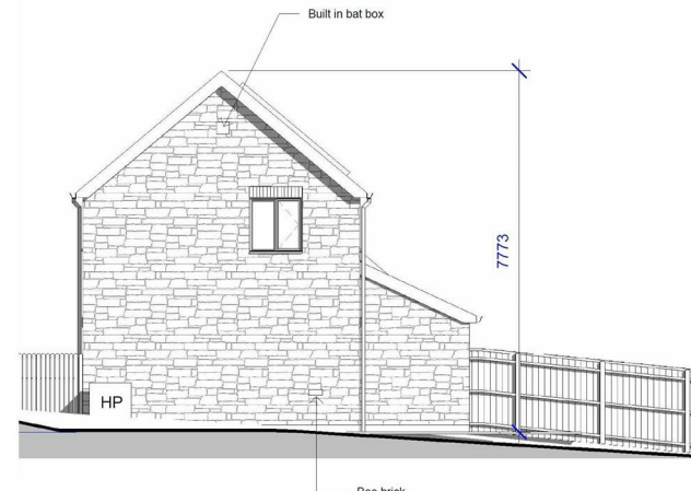
4 South West Elevation 1 : 100
