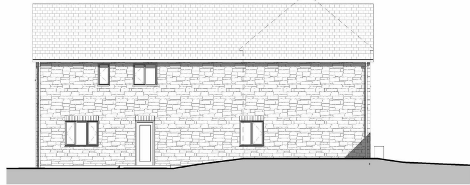
5 Plot 1 NW Elevation 1 : 100
