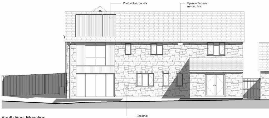
3 South East Elevation 1 : 100
