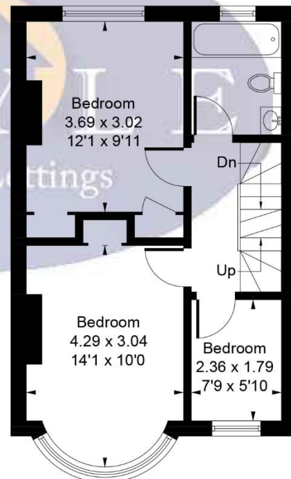
First Floor 39.98 sq m / 430 sq ft
