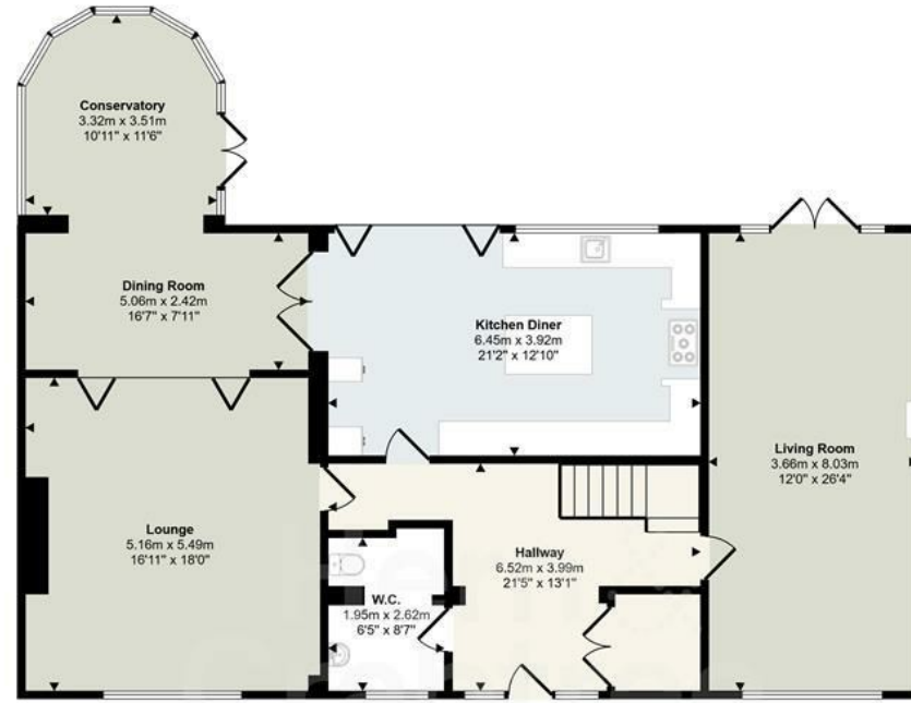
First Floor Approx 137 sq m / 1474 sq ft
