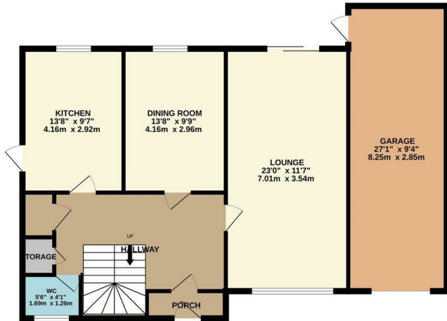
GROUND FLOOR 1015 sq.ft. (94.3 sq.m.) approx.
