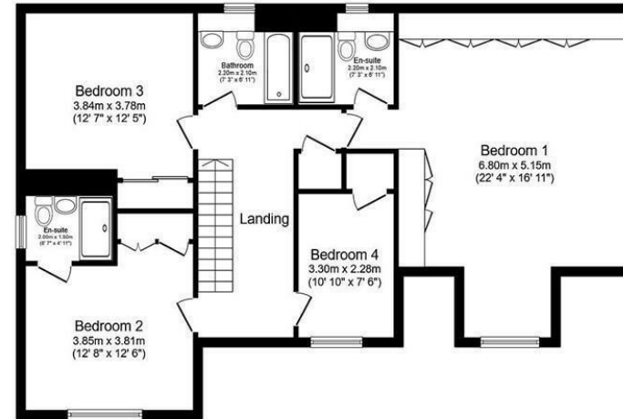
First Floor Floor area 104.1 sq.m. (1,121 sq.ft.)
