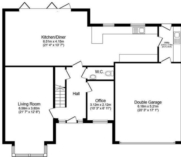
Ground Floor Floor area 128.5 sq.m. (1,383 sq.ft.)
