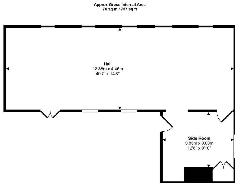
Floorplan
