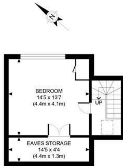
SECOND FLOOR GROSS INTERNAL FLOOR AREA WITH EAVES STORAGE 320 SQ FT FLOOR AREA WITHOUT EAVES STORAGE 252 SQ FT
