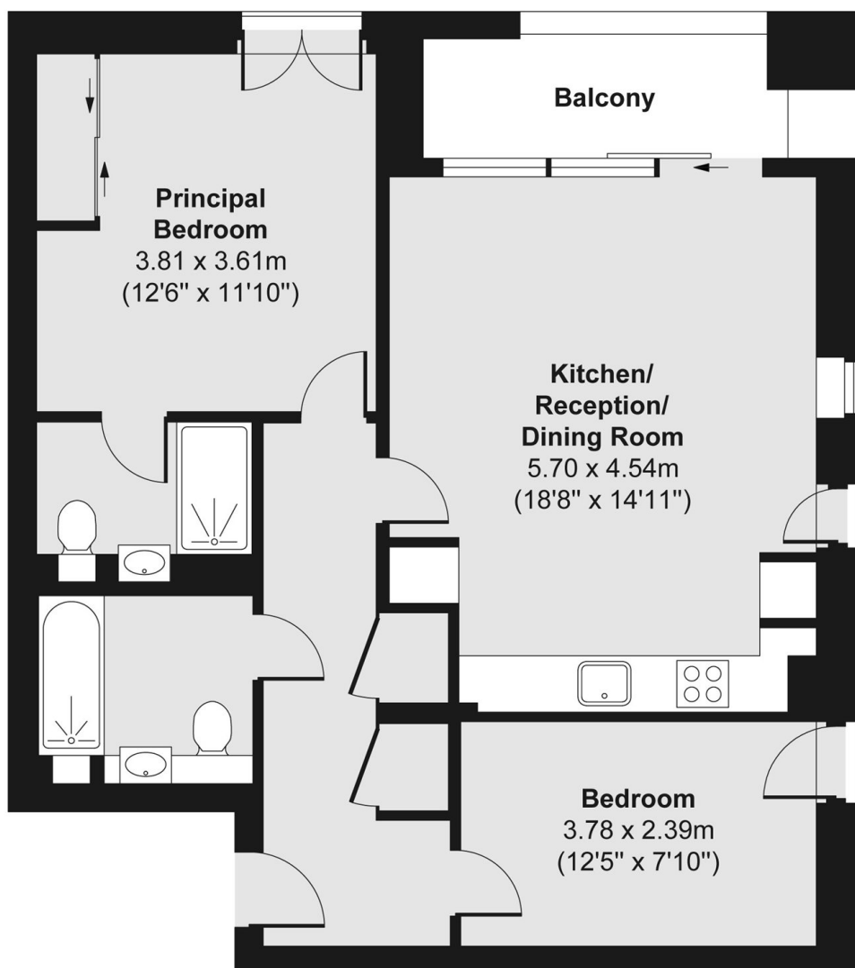
First Floor
