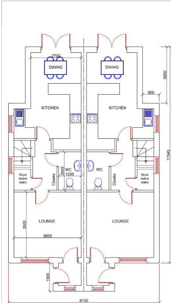
PROPOSED GROUND FLOOR PLAN Scale 1/50
