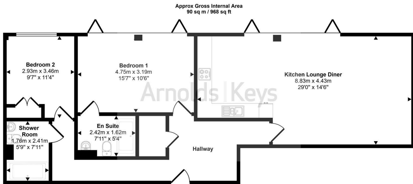
Floorplan
