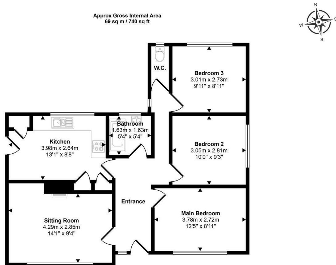
Floorplan
