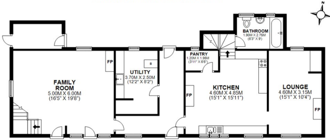
GROUND FLOOR APPROX. 84.6 SQ. METRES (911.0 SQ. FEET)
