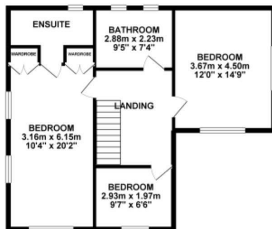
1ST FLOOR 64.81 sq. m. ( 697.61 sq. ft. )
