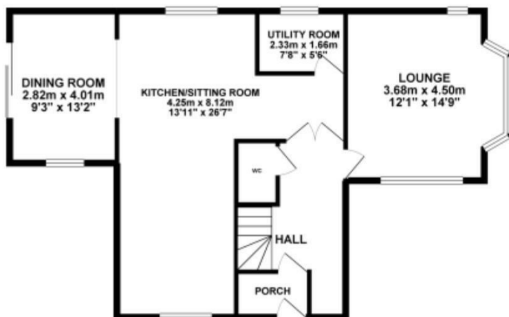
GROUND FLOOR 77.63 sq. m. ( 835.59 sq. ft. )
