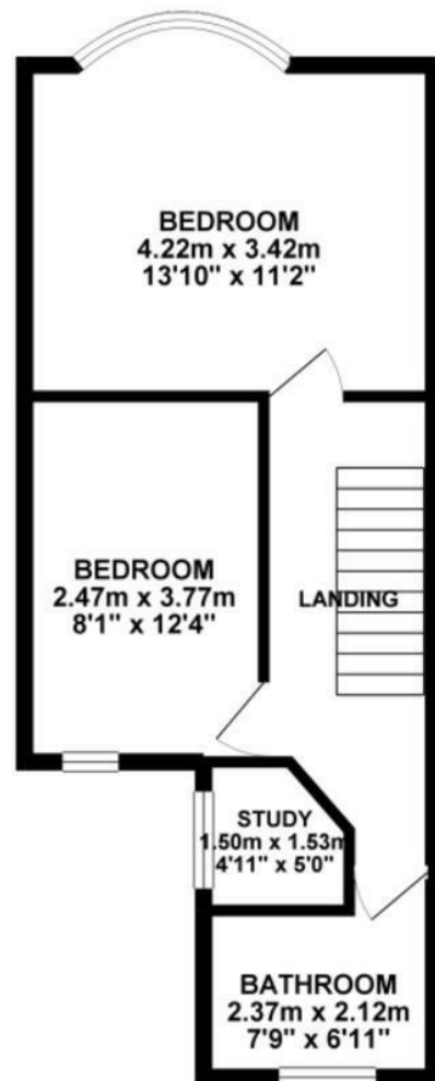
1ST FLOOR 38.75 sq. m. ( 417.15 sq. ft. )
