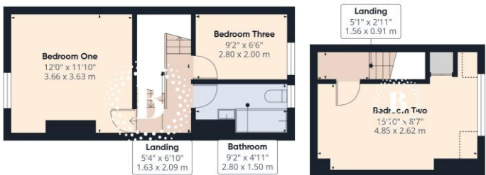
Floor 2
