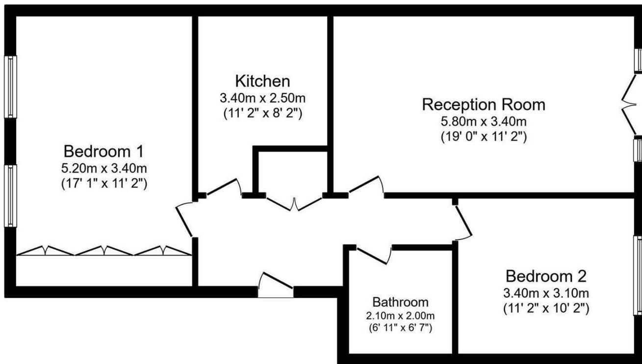
Floor Plan
