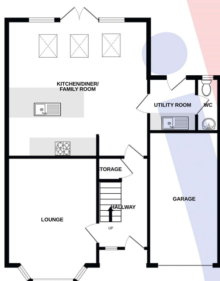
GROUND FLOOR 817 sq.ft. (75.9 sq.m.) approx.
