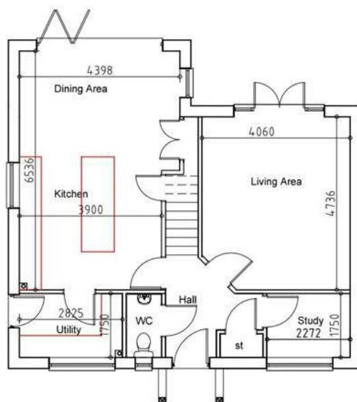
Plot 2 Ground Floor Plan Total Area - 135m sq/1453sq ft
