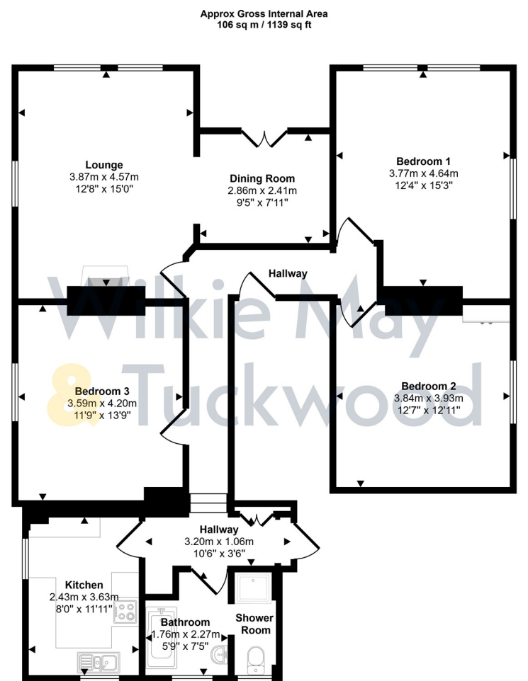
Floorplan
