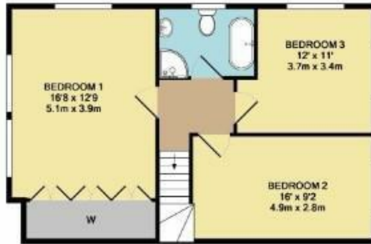
1ST FLOOR APPROX. FLOOR AREA 631 SQ.FT. (58.6 SQ.M.)
