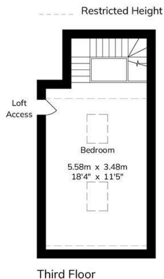
Third Floor
