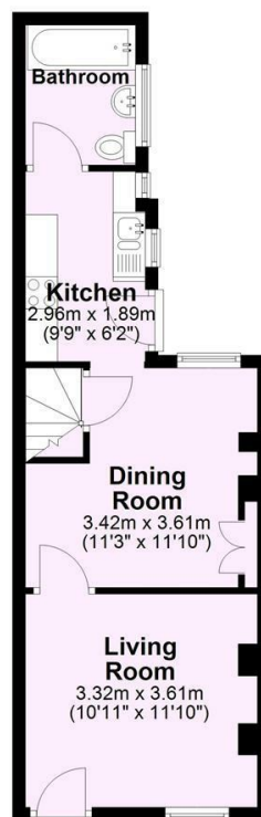
Ground Floor Approx. 34.5 sq. metres (371.6 sq. feet)
