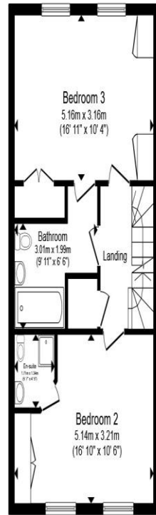
Second Floor
