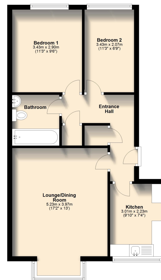
Top Floor Approx. 56.3 sq. metres (606.2 sq. feet)
