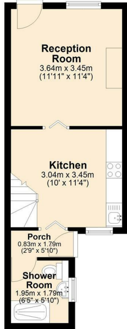
Ground Floor Approx. 28.7 sq. metres (309.2 sq. feet)
