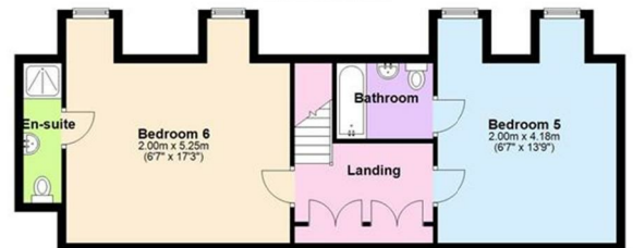
Second Floor Approx. 62.1 sq. metres (668.9 sq. feet)
