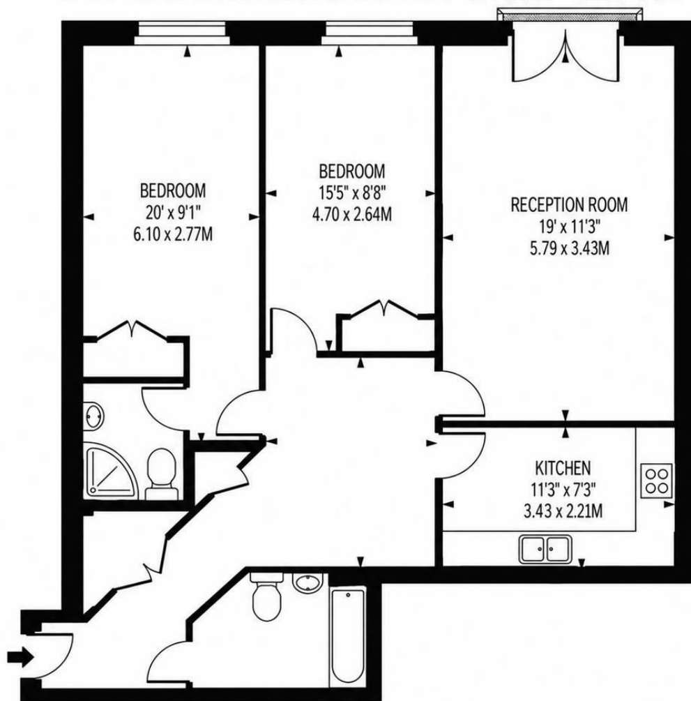
FIRST FLOOR
