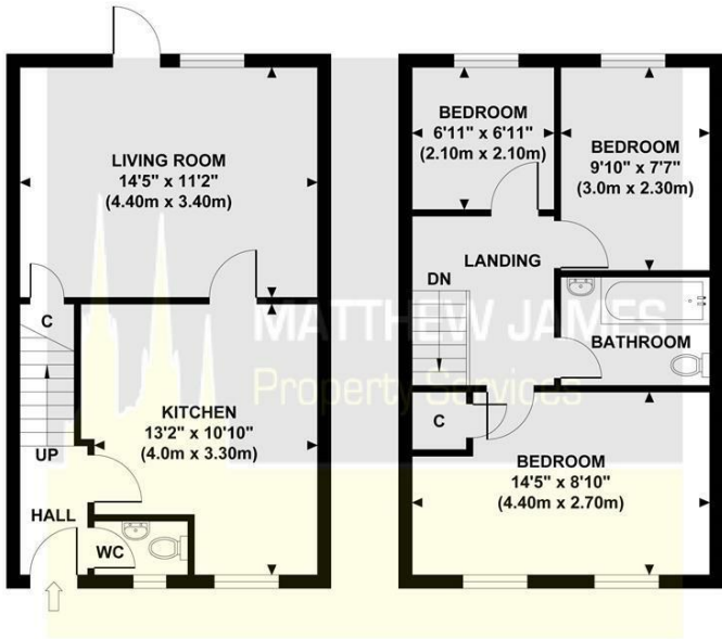
GROUND FLOOR GROSS INTERNAL FLOOR AREA 350 SQ FT
