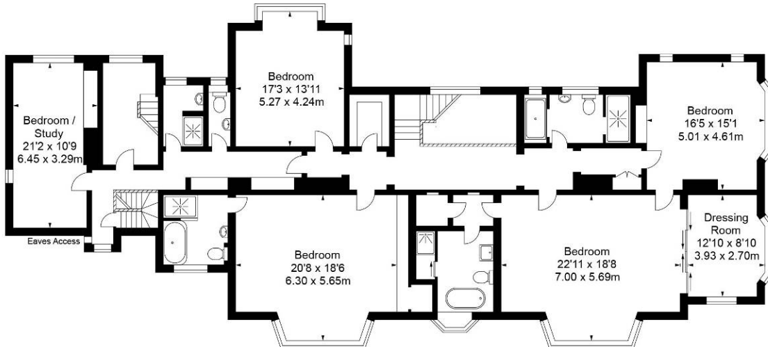
First Floor
