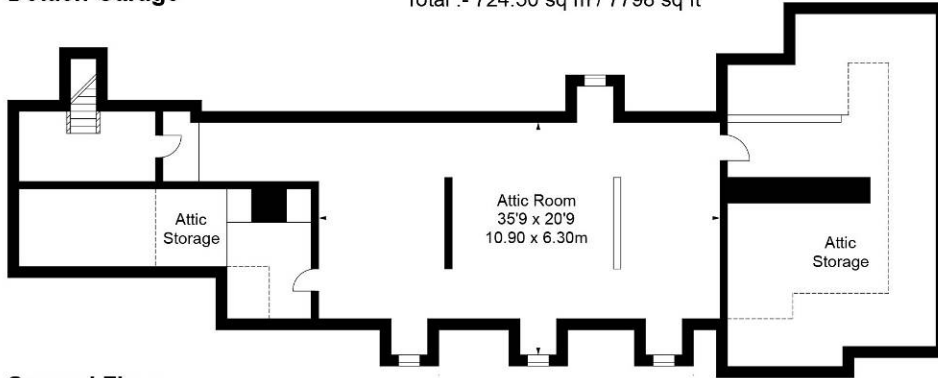
Second Floor
