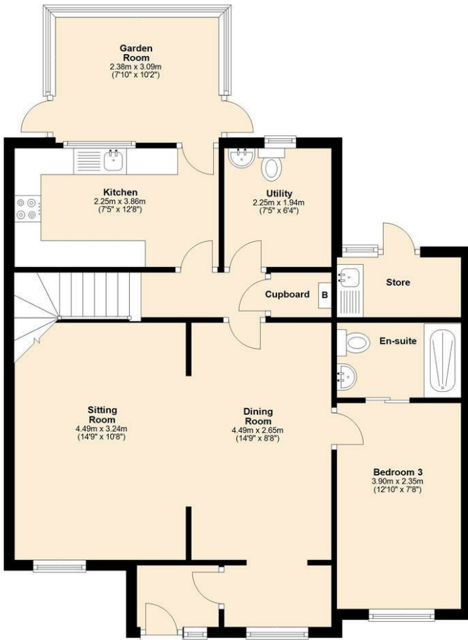
Ground Floor Approx. 74.8 sq. metres (805.3 sq. feet)
