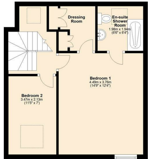
First Floor Approx. 38.6 sq. metres (415.8 sq. feet)
