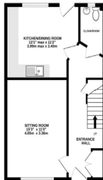
GROUND FLOOR 482 sq.ft. (44.3 sq.m.) approx.
