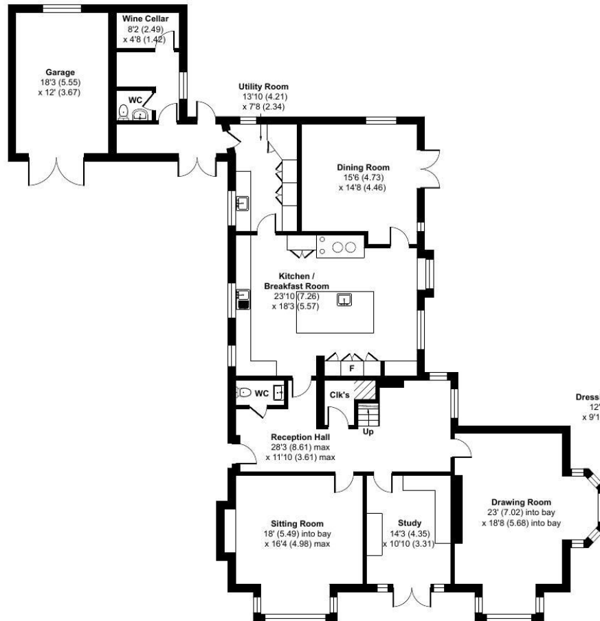
GROUND FLOOR
