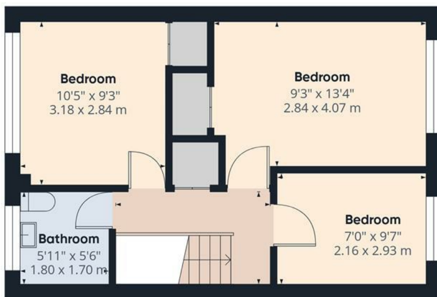
Floor 1
