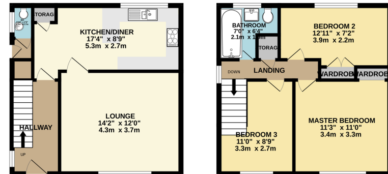
GROUND FLOOR 782 sq.ft. (72.6 sq.m.) approx.
