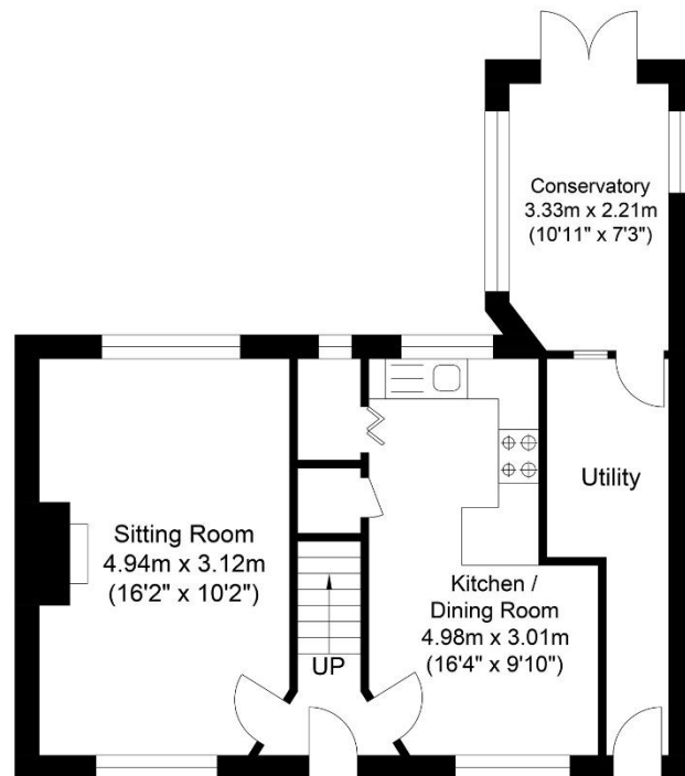
Ground Floor Approximate Floor Area 488.25 sq ft (45.36 sq m)
