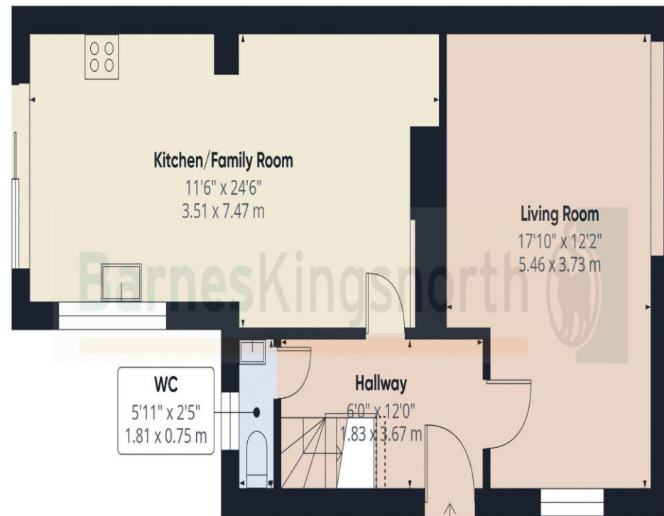
Floor 0
