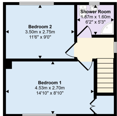
First Floor Approx 31 sq m / 336 sq ft
